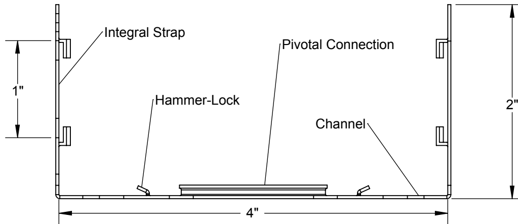
Sectional View
